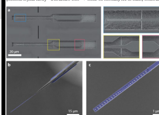
Top left: Scanning electron micrograph top view of the fabricated device on a silicon substrate chip. Right: Zoom-ins of the boxed regions. b) False colour scanning electron microscope image showing the wave flume and photonic crystal cavity. c) False colour scanning electron microscope image showing the photonic crystal cavity at the end of the device. The silicon waveguide is around 500 nm wide and 220 nm thick. APRIL 2025, PALCO ZHONG
